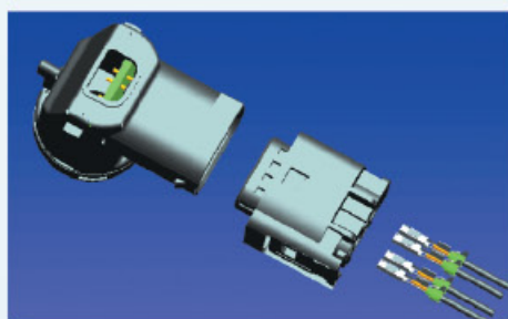
Sensor Connector for Driveless Cars
